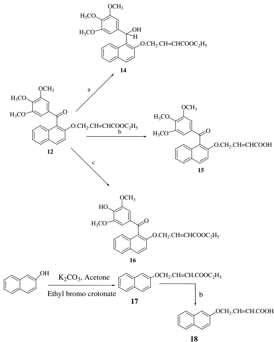
Scheme 2. Reagents and conditions: (a) NaBH 4 /MeOH, 40–50 °C, 89%; (b) 10% KOH in 10 mL MeOH–H 2 O = 3:1, 60 °C, 1 h, 82%; (c) AlCl 3 –DCM, rt, 62%.
