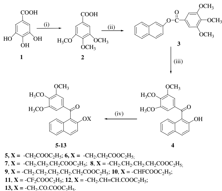
Scheme 1. Reagents and conditions: (i) \text{Me}_2\text{SO}_4/\text{KOH} , 10–20 °C for 30 min, then reflux for 3 h, 76%; (ii) DCC/DMAP, DCM, 4 h, 71%; (iii) \text{AlCl}_3 neat, 120–130 °C, 31%; (iv) different ethyl bromo esters, dry acetone, \text{K}_2\text{CO}_3 , 58–89%.
